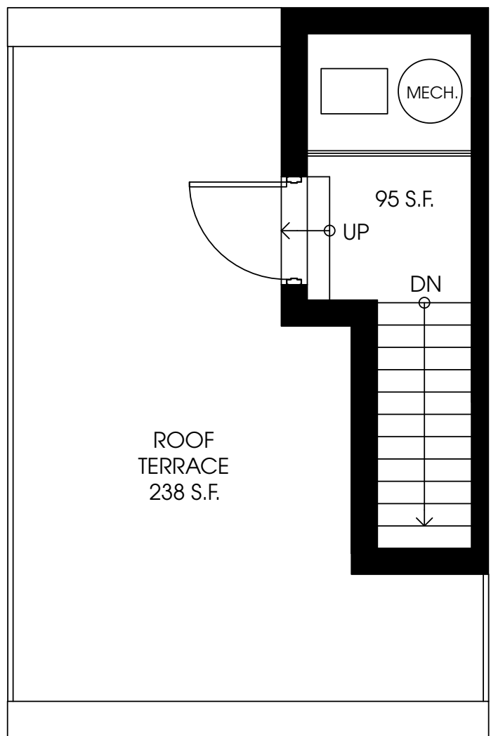
ROOF TERRACE
